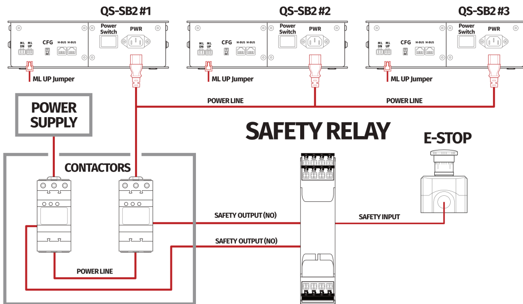
Example application of power line contactors and E-STOP button:
